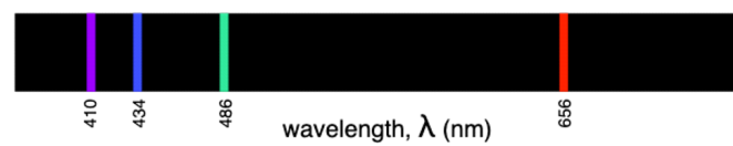
Hydrogen Emission Spectrum
